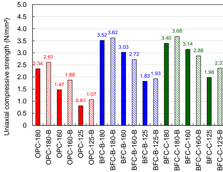
Figure 5. Uniaxial compressive strength results.
