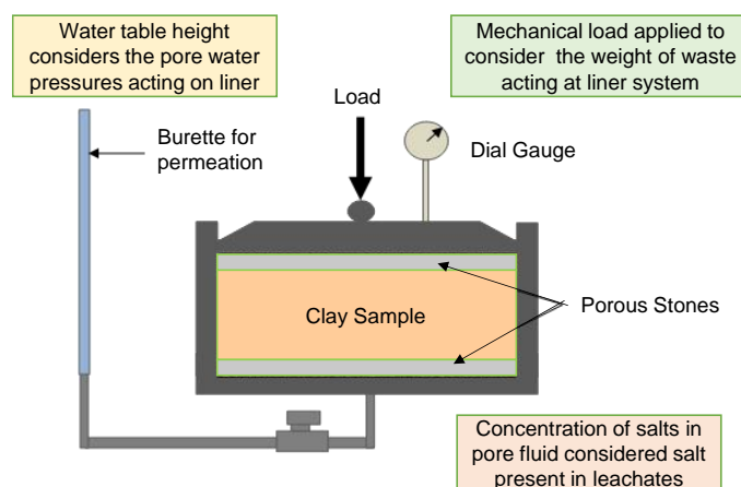
Figure 1. Schematic diagram for permeation set-up under loading conditions.
