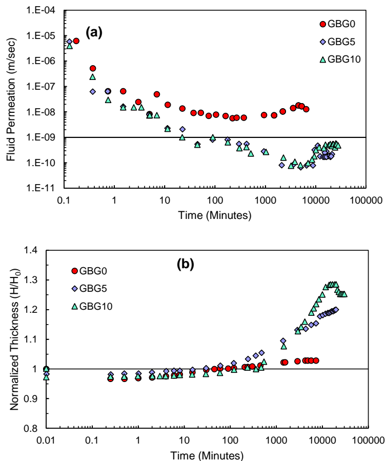
Figure 4. Temporal variations of (a) fluid permeation; and (b) normalized thickness with guar gum amended GB using 0.5M CaCl 2 as pore-fluid under 50 kPa mechanical loading.
